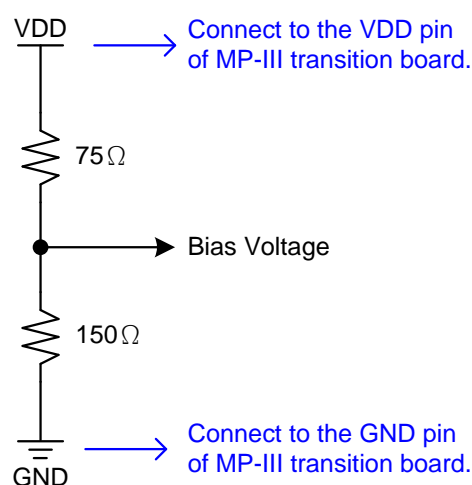
Bias Circuit:
